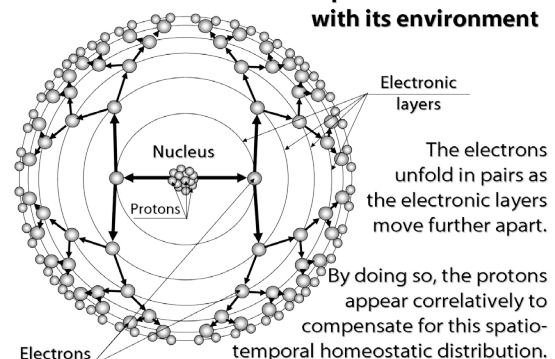
Genesis of a stable atom prior to interaction with its environment
